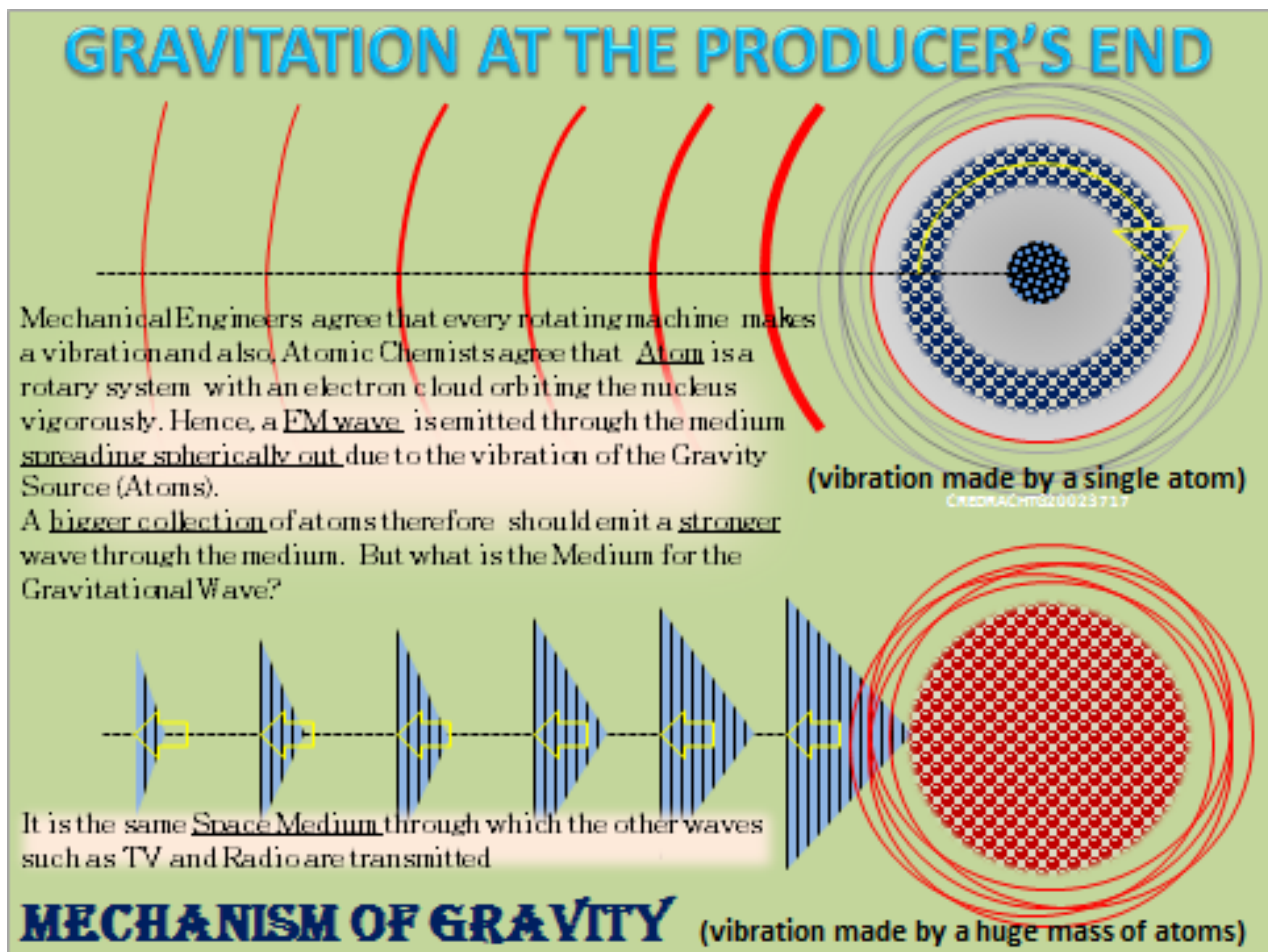
Figure-06 (Origin of gravitational waves)
