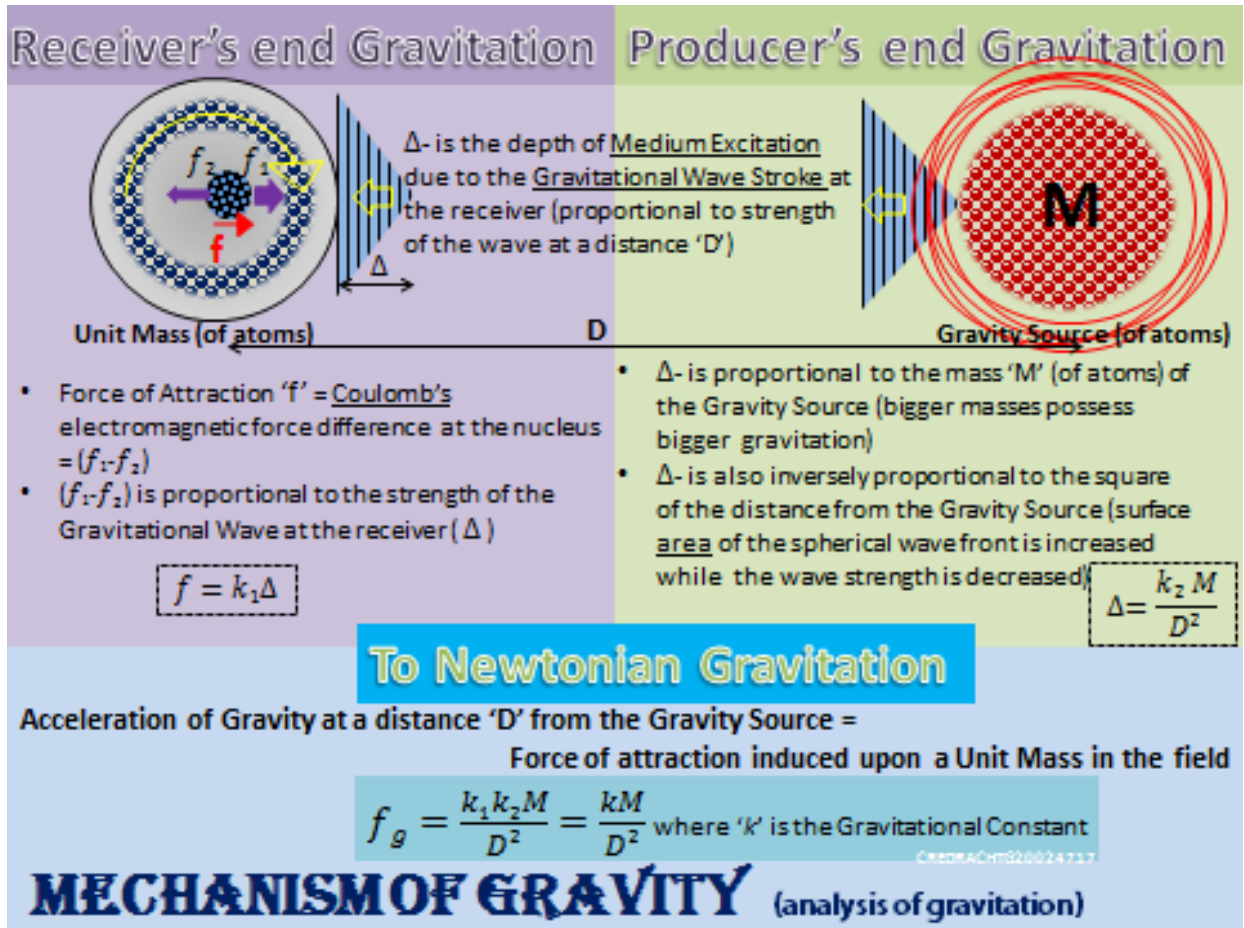
Figure-08 (Analysis to prove Newtonian Gravity by the wave concept)
