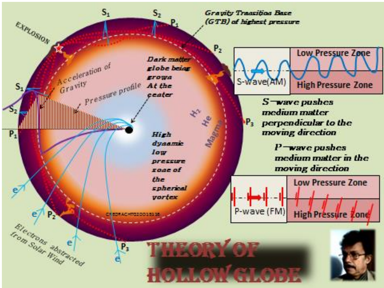
Figure-16 (The alternative model of the Globe)
