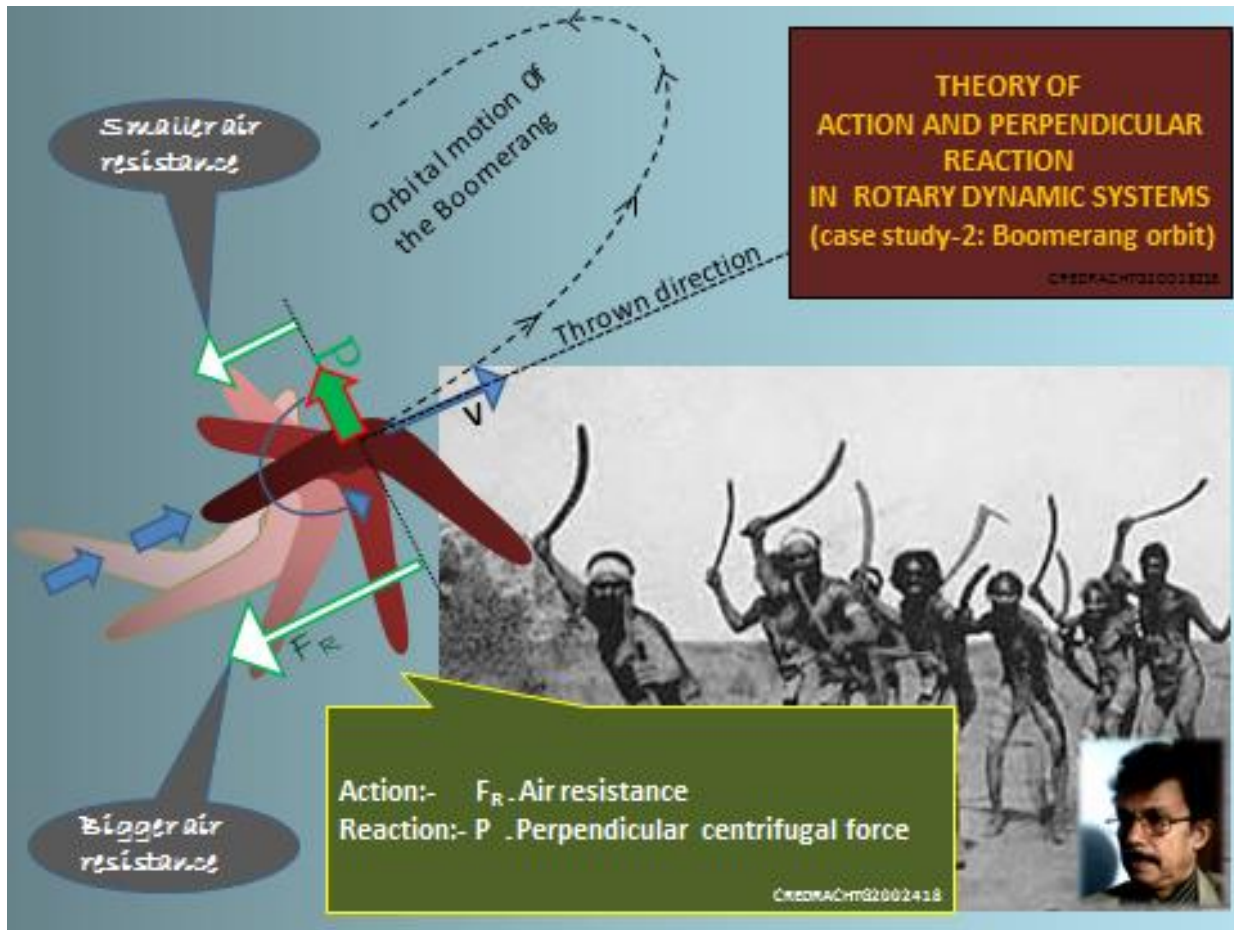
Figure-03 (Demonstration of the orbital motion of a boomerang)
