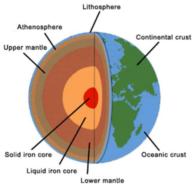
Figure-12 (The conventional Earth Structure)
