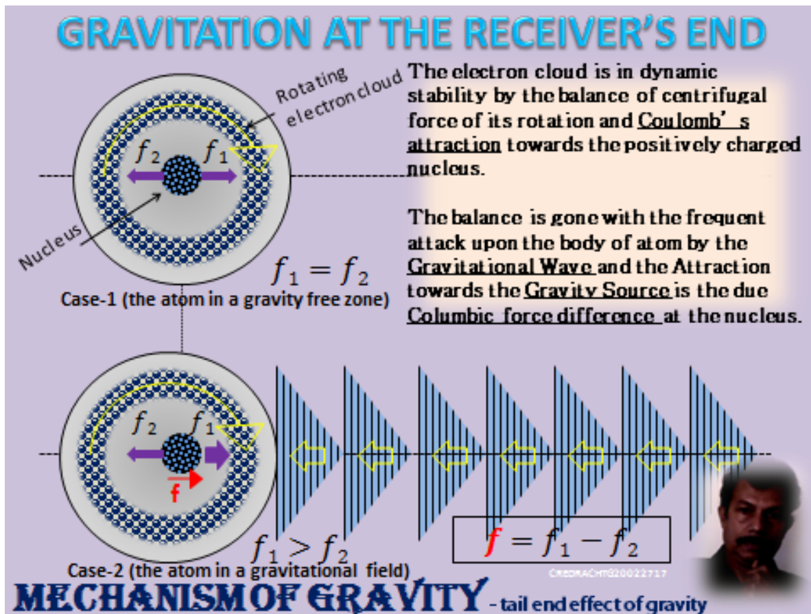
Figure-07 (Demonstration of how atomic bodies are succumbed to Gravity)
