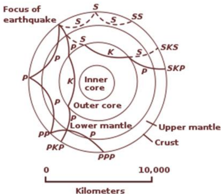
Figure-13 (Demonstration of how seismic waves are returned defining layers)
