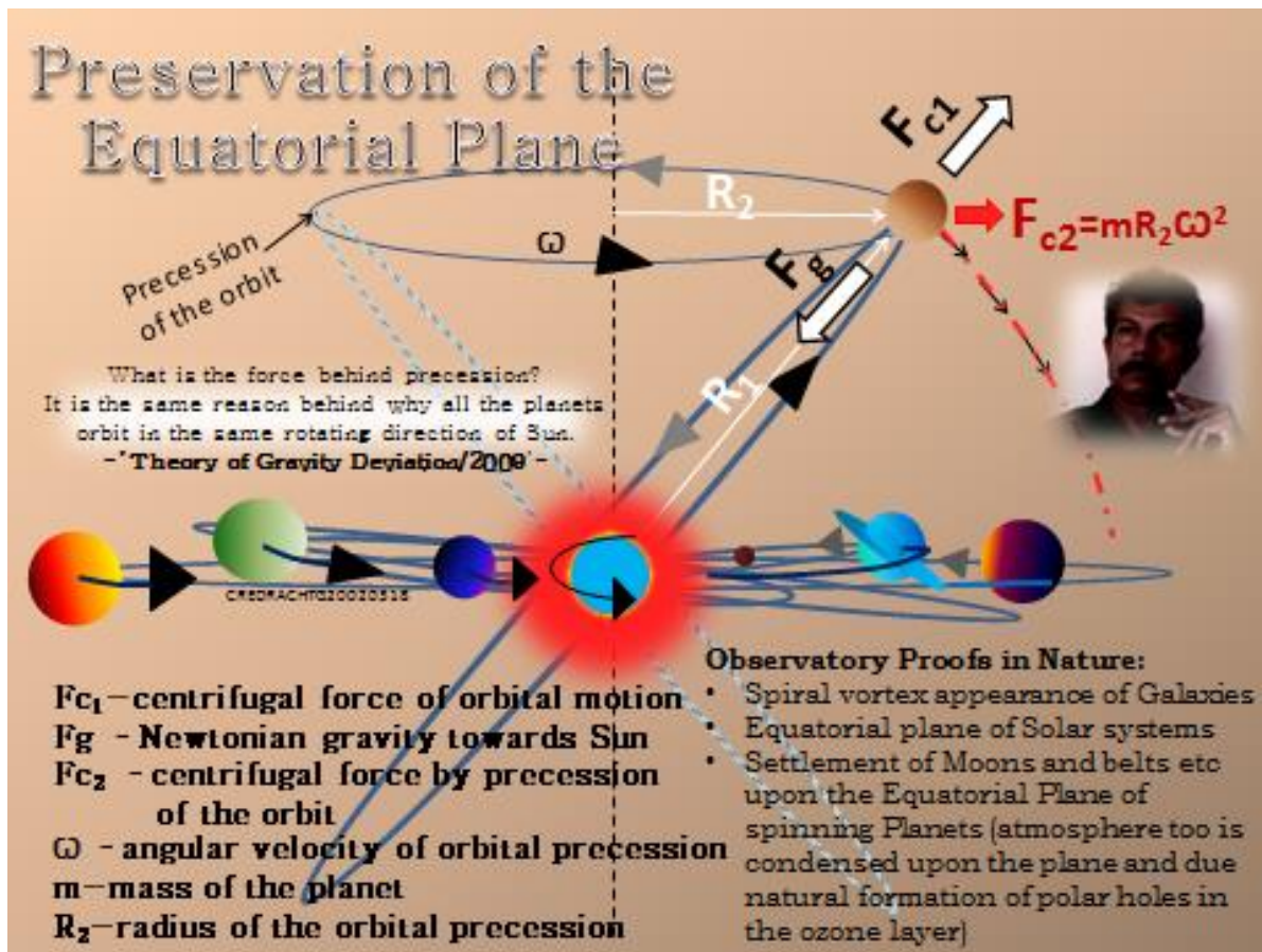
Figure-11 (Demonstration of the theory of equatorial plane)
