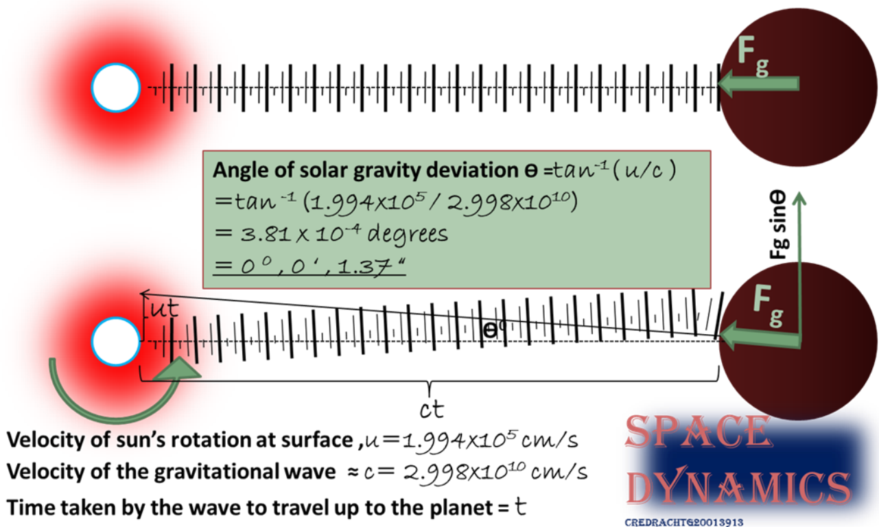
Figure-09 (Demonstration of the theory of Gravity Deviation)
