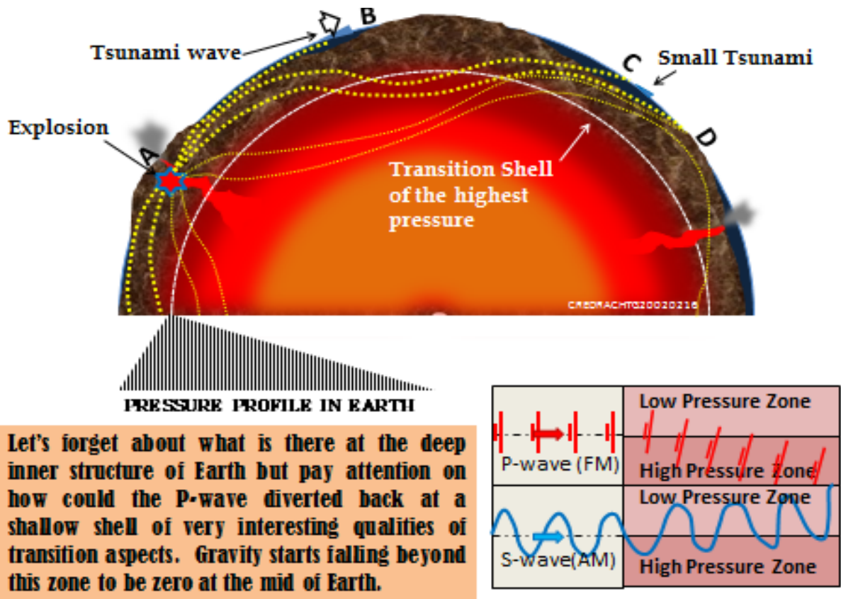
Figure-15 (The realistic way of Seismic P-wave propagation in side of Earth)
