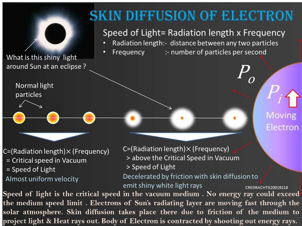
FIGURE-01 (Light & Heat rays by Skin Diffusion of Electron)
