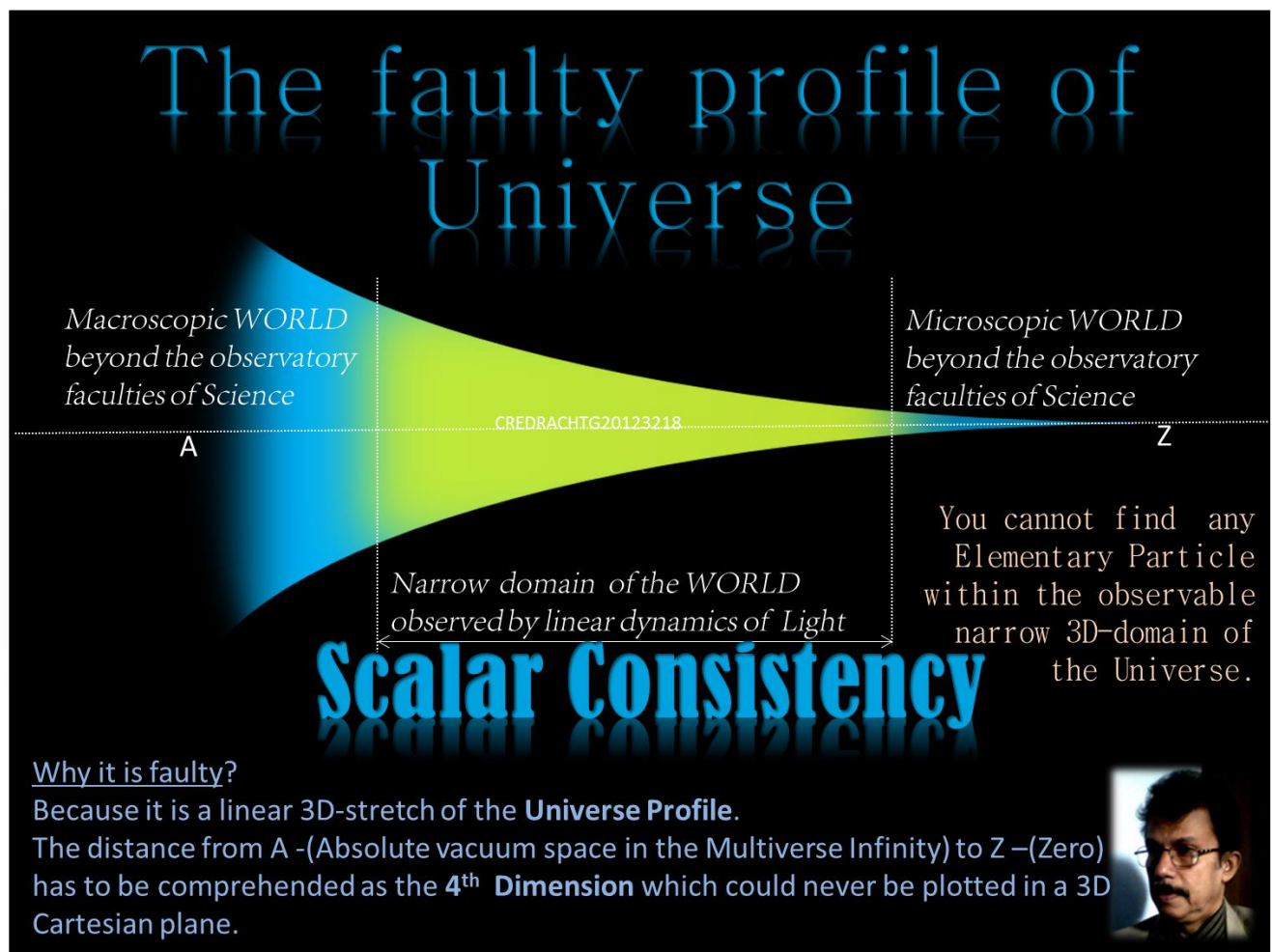
FIGURE-08(the faulty 3D-stretch of the Universe)
