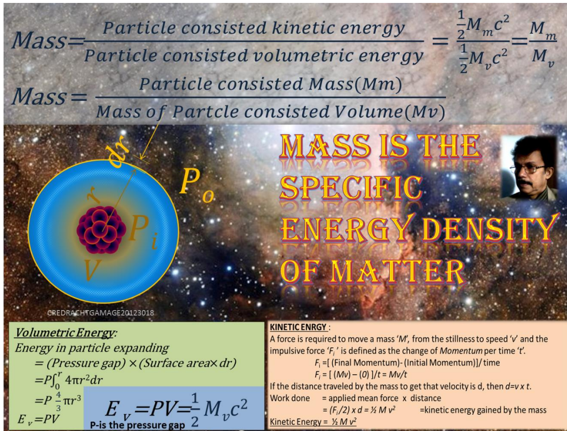
FIGURE-06 (Mas of Matter-as abstracted from 'Scalar Consistency of Matter')
