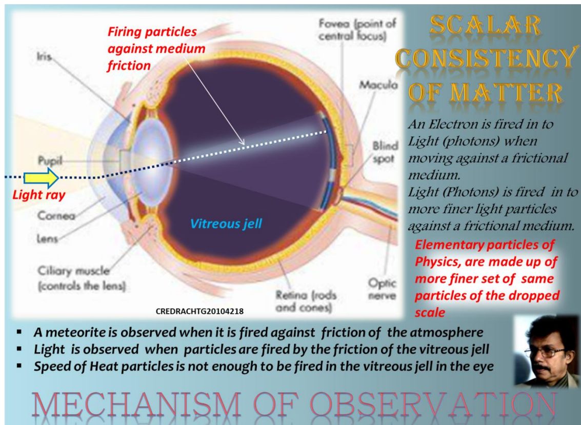
FIGURE-7 (Demonstration of the mechanism of Observation)
