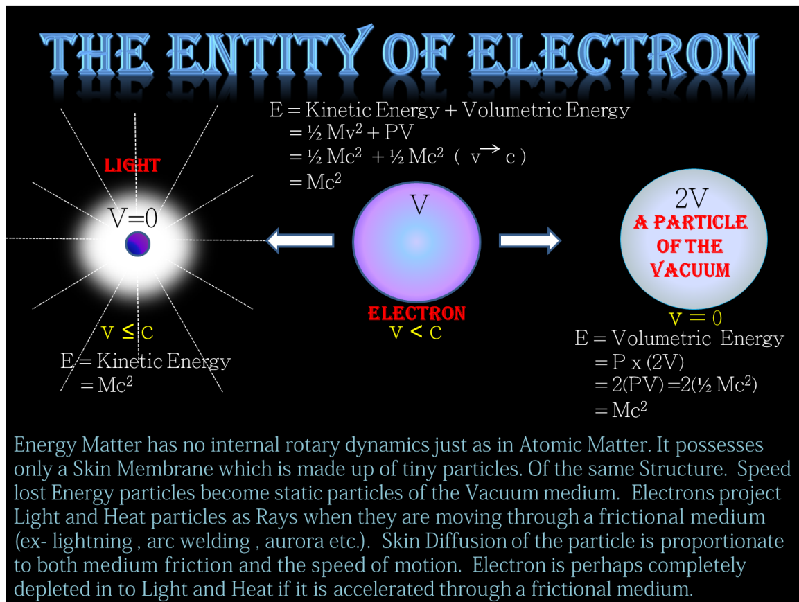
FIGURE-03 (demonstration of end entities of Energy Matter)
