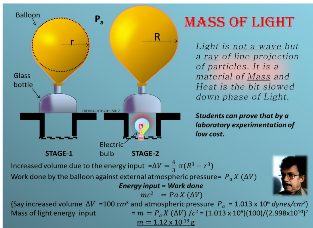
FIGURE-05 (Typical exhibition for Mass of Light)
