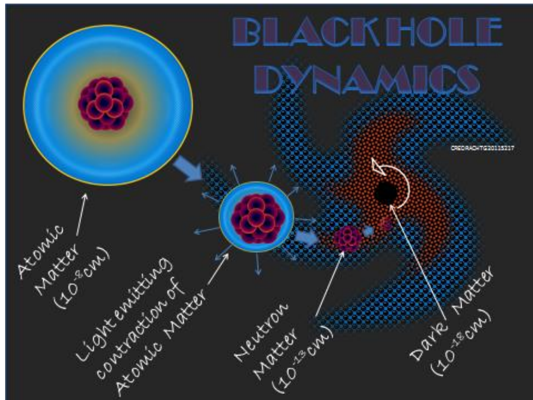
FIGURE-03(CONTRACTING MECHANISM OF BLACK HOLE)
