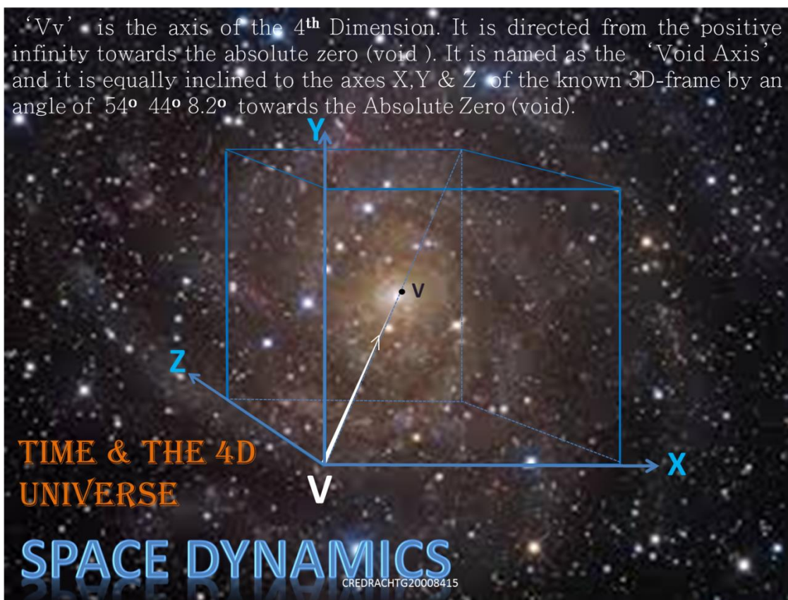
FIGURE-02 (DIMONTRATION OF THE 4 TH DIMENSION-abstracted from 'Time & The 4D Universe'/2015)
