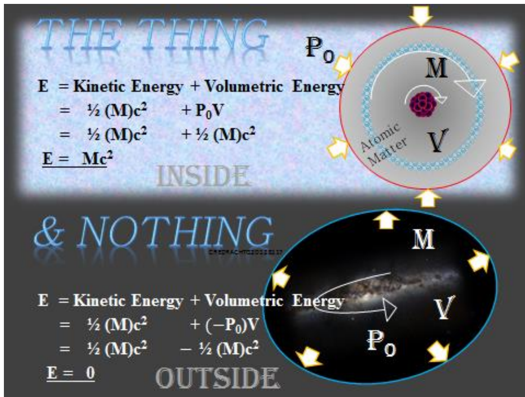
FIGURE-05(NOTHING REMAINS AS MATTER IN THE OUTSIDE)
