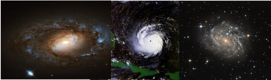
FIGURE-01(A hurricane among Galaxies)
