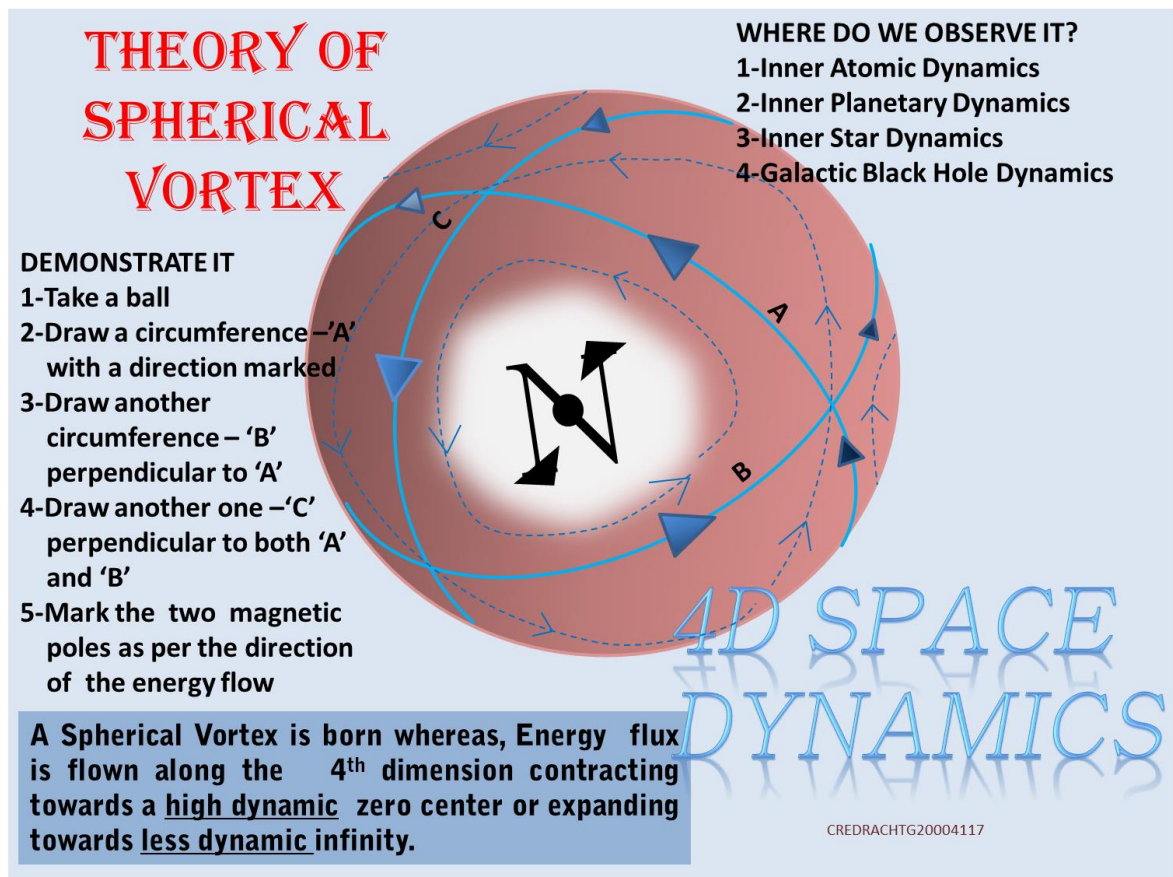
FIGURE-01 (DEMONSTRATION OF THE SPHERICAL VORTEX)
