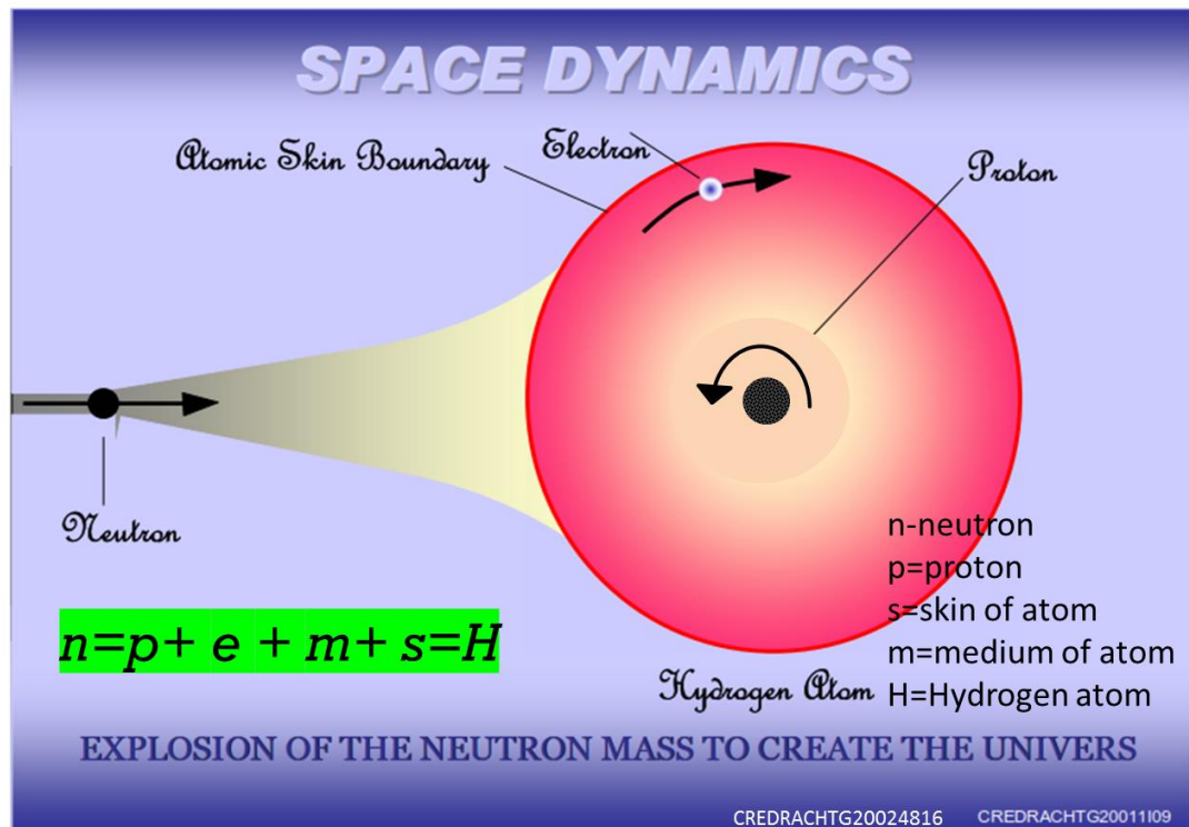
Figure-04(abstrated from 'Space Dynamics-V1'/2009)
