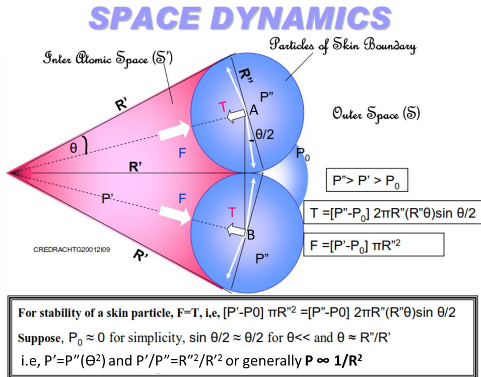
Figure-06 (abstracted from ‘Space Dynamics-V1/2009’) Projected particles behave as light & heat in rays and the mother electron is worn out in mass and energy as well. Above mathematical deduction also gives an important relation about energy particles such as; Pressure in an energy particle is inversely proportionate to square of the radius.
