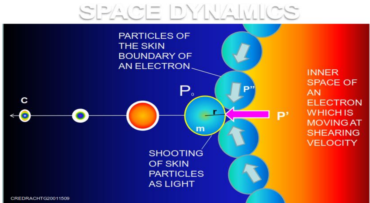
Figure-05(abstrated from 'Space Dynamics-V1'/2009)
