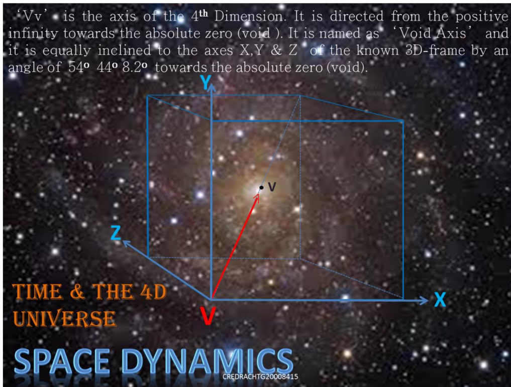
Figure-21 (abstracted from 'Space Dynamics-V8/2015)
