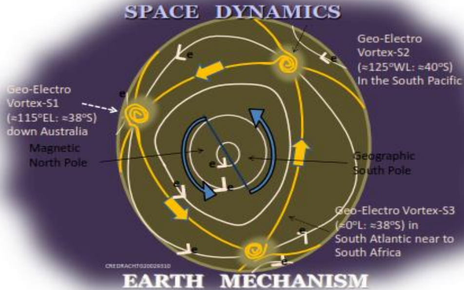
Figure-12 (abstracted from 'Earth Mechanism/2010)
