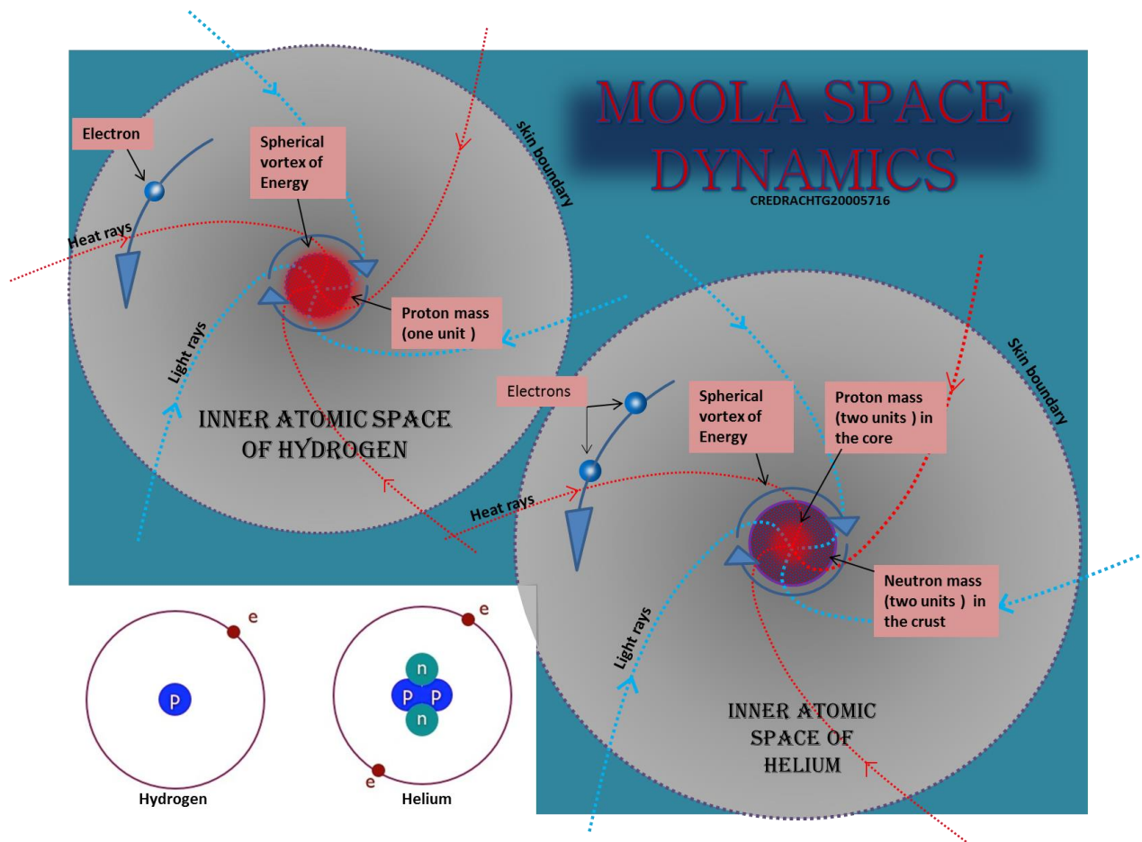
Figure-13 (Inner structure of Hydrogen and Helium)
