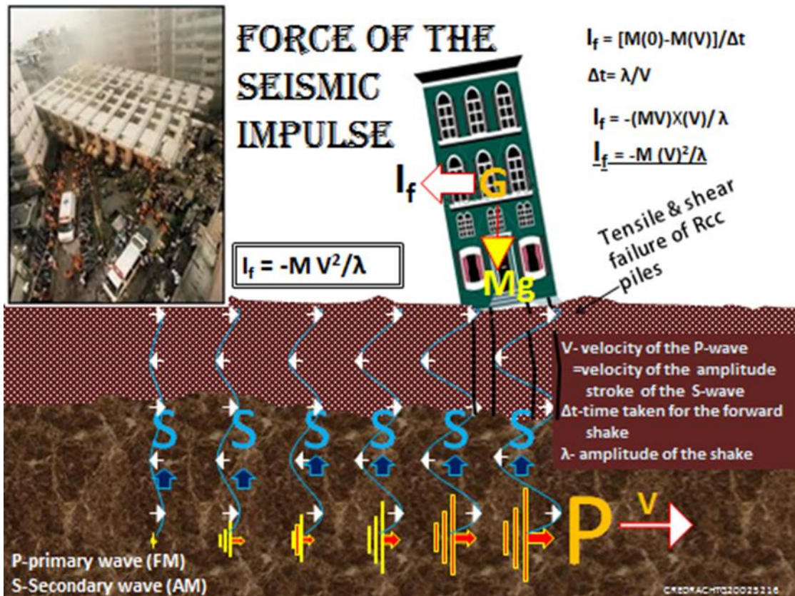
Figure-07 (abstracted from 'Theory of seismic impulse'/2016)
