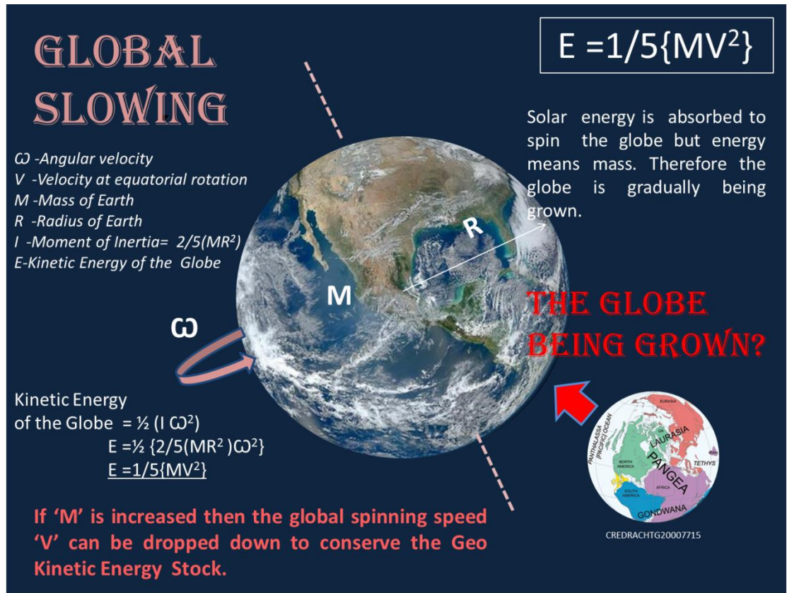
Figure-19(Abstracted from "Theory of Solar mass Transplantation /2015')
