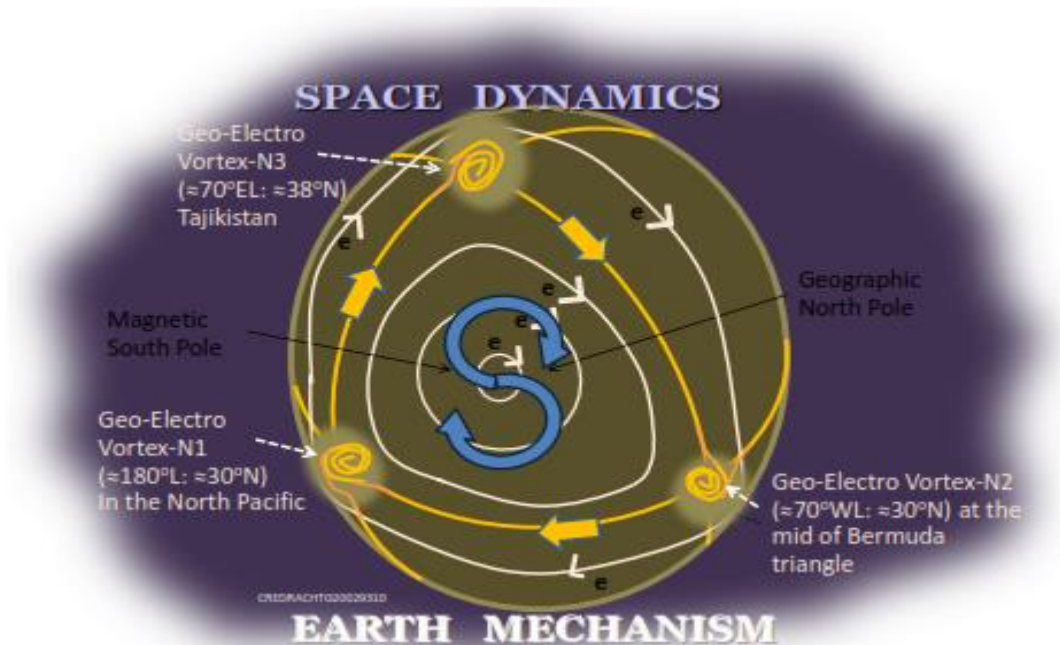
Figure-11 (abstracted from 'Earth Mechanism'/2010)
